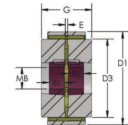
FIGURE 11 INTERNAL TAPER-LOCK
