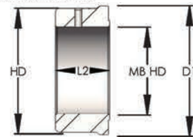
FIGURE 15 HEAVY DUTY RING HUB
