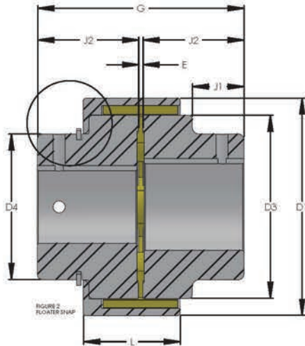
FLOATER SNAP
