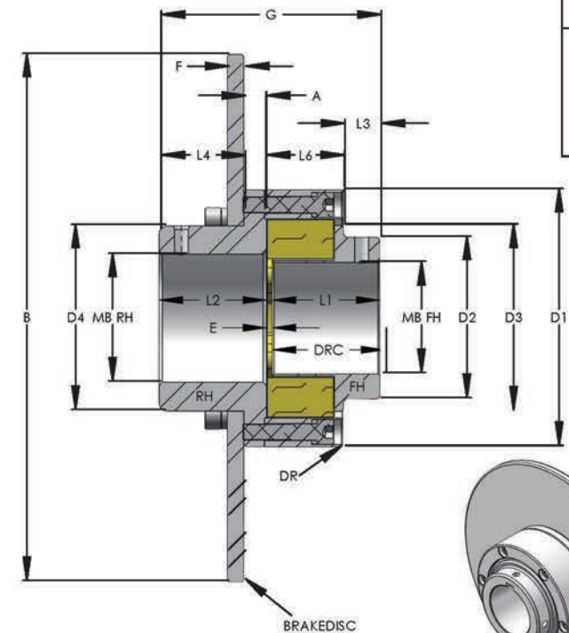
FIGURE 22 BRAKEDISC
