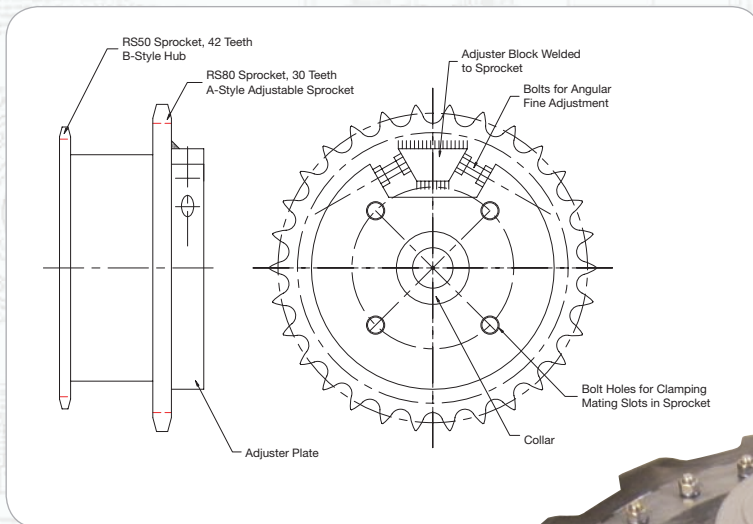
Custom Adjustable Roller Chain Sprocket Assembly
