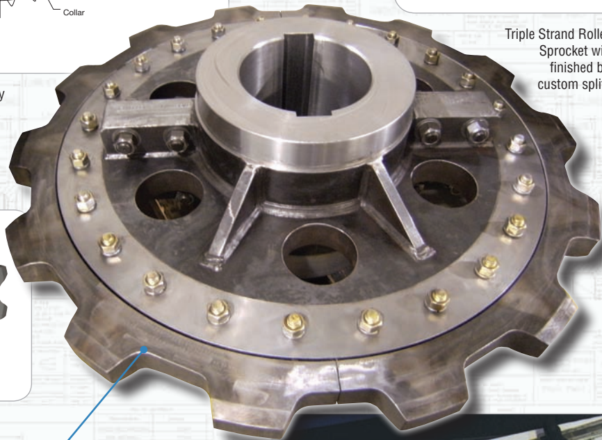
Custom Adjustable Roller Chain Sprocket Assembly
